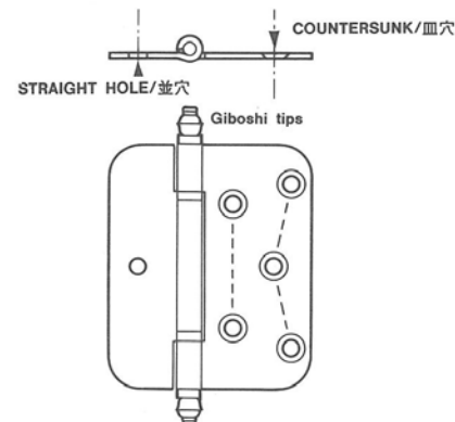
隅丸・ギ星付・片巾広/ONE WIDE LEAF with ORNAMENTAL TIPS.
