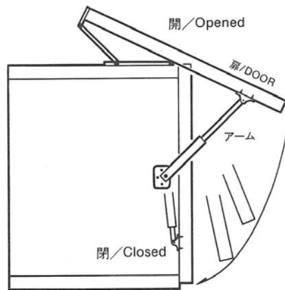
■ 側断面/SIDE VIEW: SECTION
