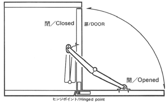
■ 側断面/SIDE VIEW: SECTION
